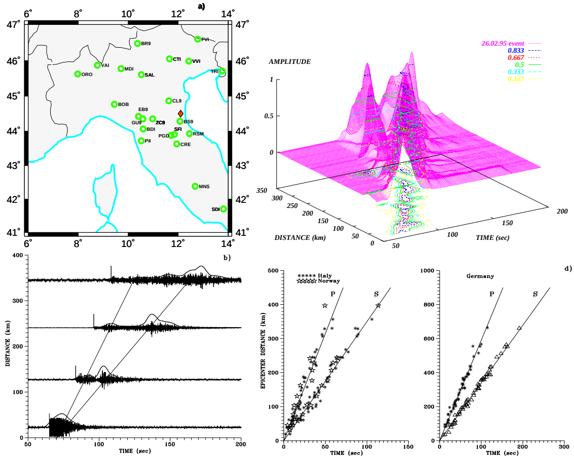
Figure 1: Example of energetic wavelet processing from stations green circles of the Italian network for an event 26.02.1995 red rhombus . b). Original waveform records and EW-envelopes. First arrivals are marked with flags c) The entire set of relevant dimensionless envelopes, ordered with respect to epicenter distances. Amplitude isolines are drawn below. Note the linear spreading of EW (c) which is typical of diffusion processes . d) P- and S-energetic wavelet travel times curves for Italian, Norwegian and German networks. The P- and S-EW maxima are automatically identified and picked at the event post-localization stage . The dispersion of maxima for the German network was essentially reduced after a brief period of 'network training'. The corresponding EW-velocities are 6.3 km/s and 3.5 km/s for Italy/Norway and 5.9 km/s and 3.4 km/s for Germany.
