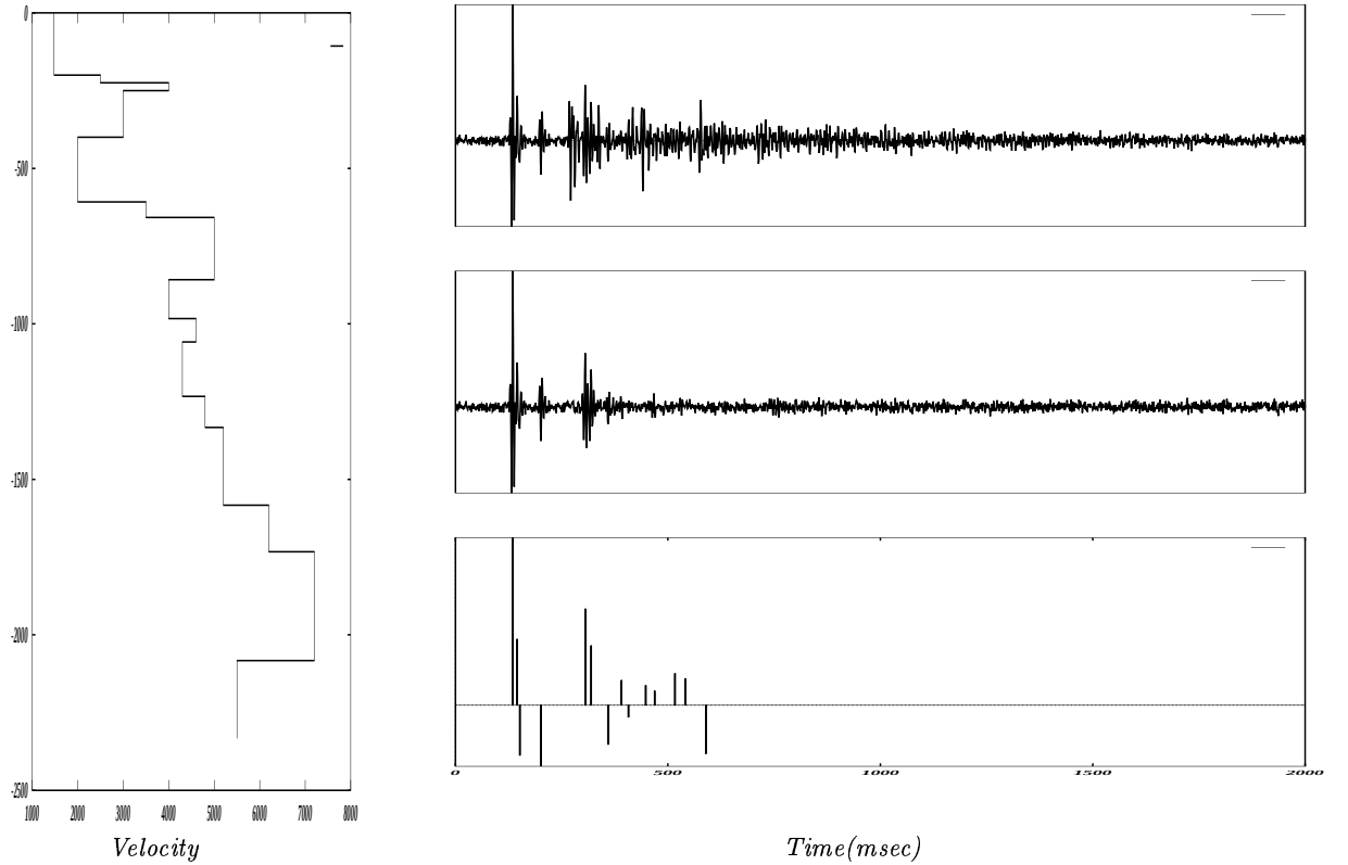
Fig. 1. The computer simulation of the marine data processing: multiple suppression with SDec -filter. Left: velocity model; right (from the top to bottom): • input record with additive noise ; • output; • true primaries of the impulse trace.
